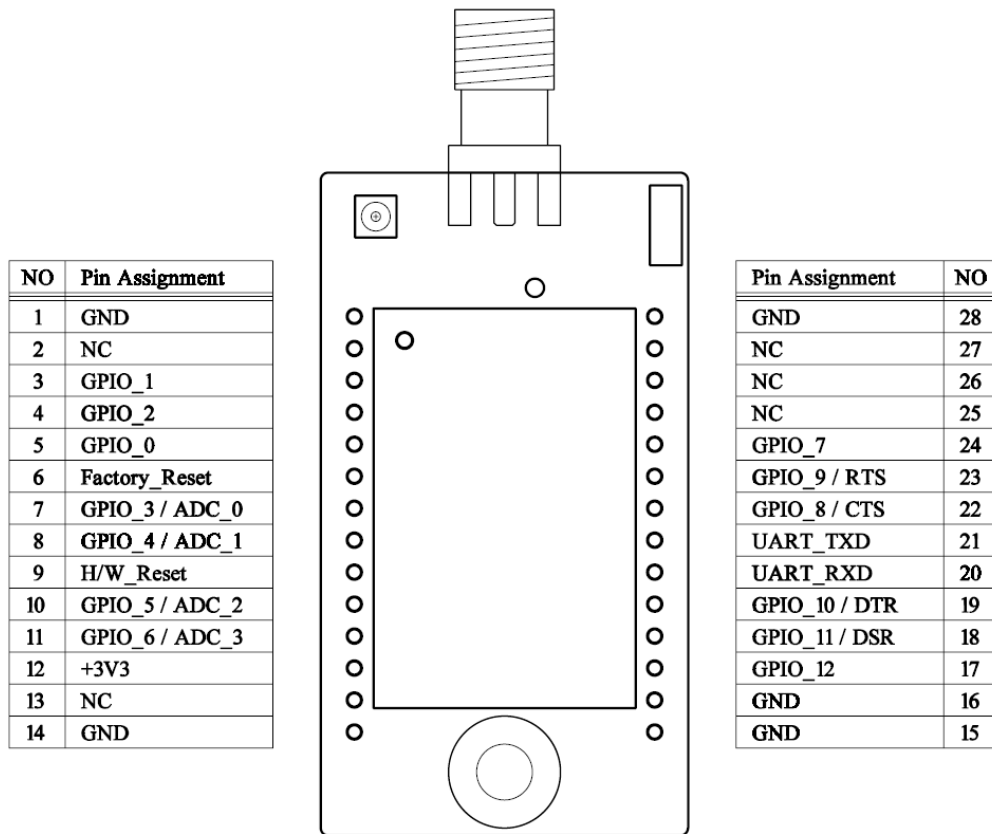
Figure 1-2 Pin Diagram
