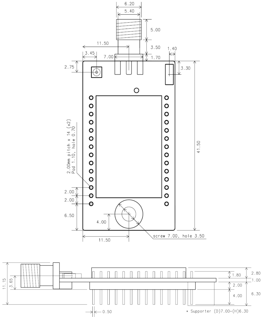
Figure 1-3 Mechanical Drawings
