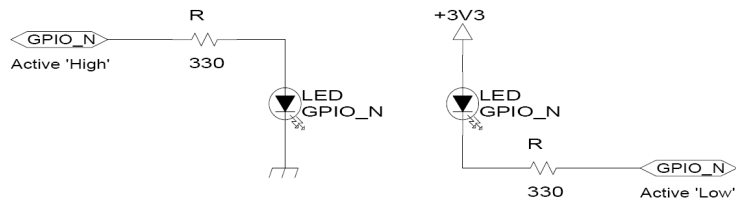
Figure 5-6 GPIO LED Output
