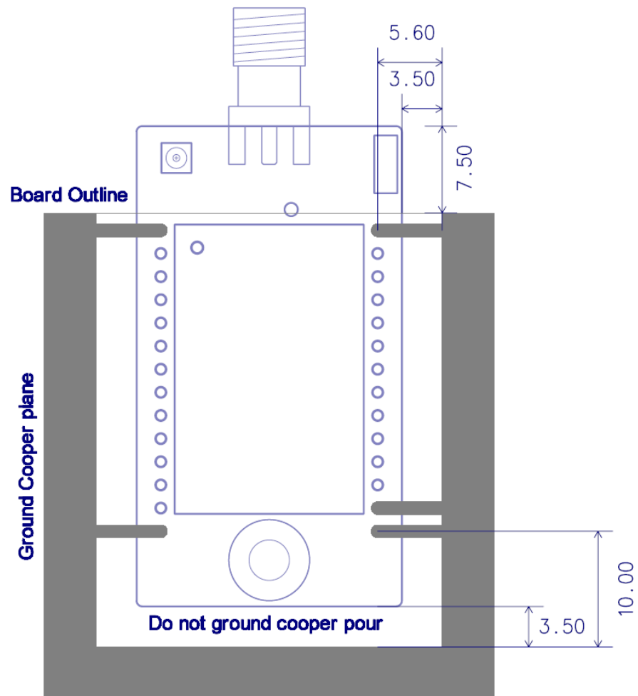
Figure 1-4 Recommended PCB Layout
